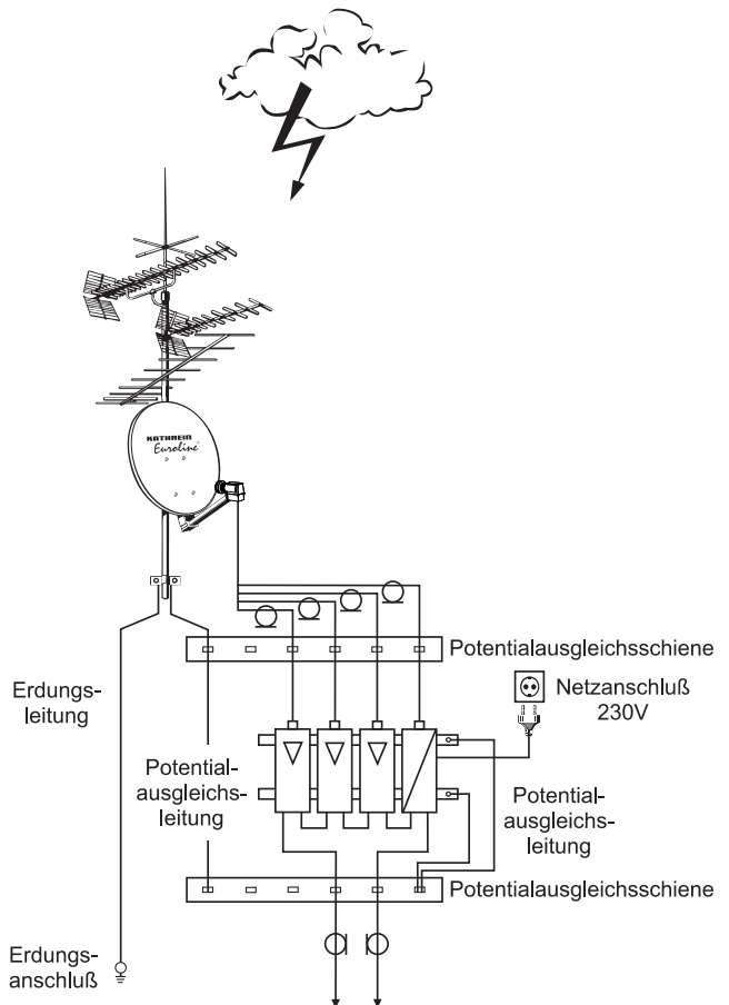
Fig. 12: Grounding of antenna
