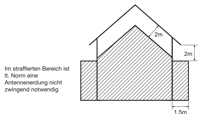
Fig. 13: Areas for antenna grounding
