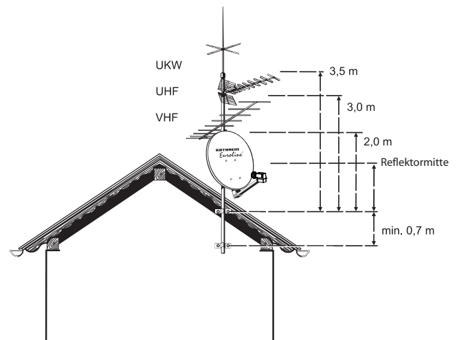
Fig. 3: Several antennas on a single antenna carrier
