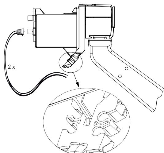
Fig. 5: Cable connection
