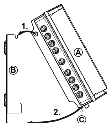
Fig. 3: Insert the head-end
