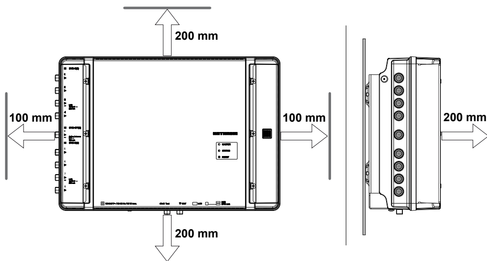
Fig. 2: Allow the necessary clearance for air circulation
